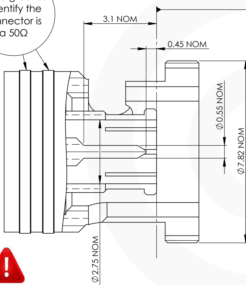
PLUG
